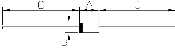
DO-204AC(DO-15)
